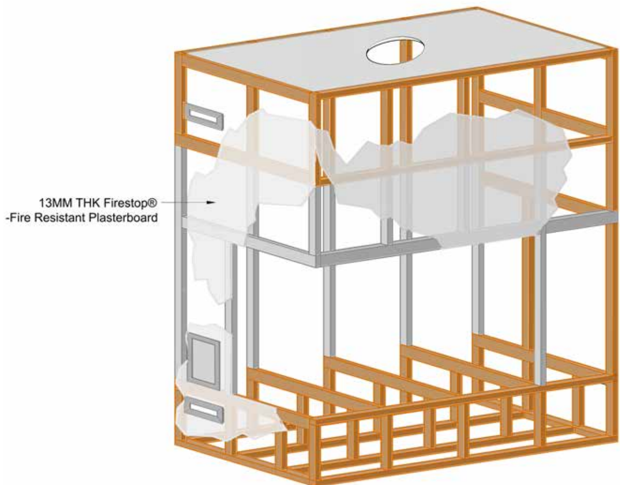
Figure 1.7 (Cladding Material)
