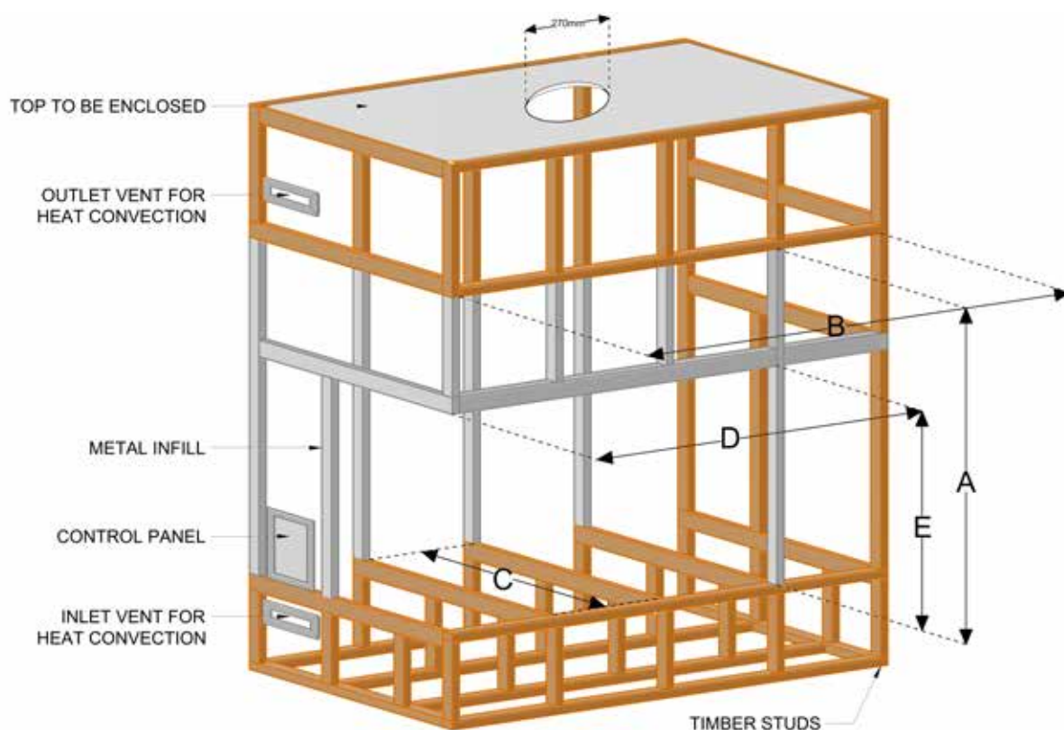
Figure 1.8 (Timber framing)
