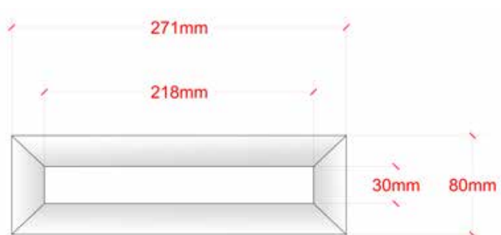
Figure 1.3 (Vent Size)
